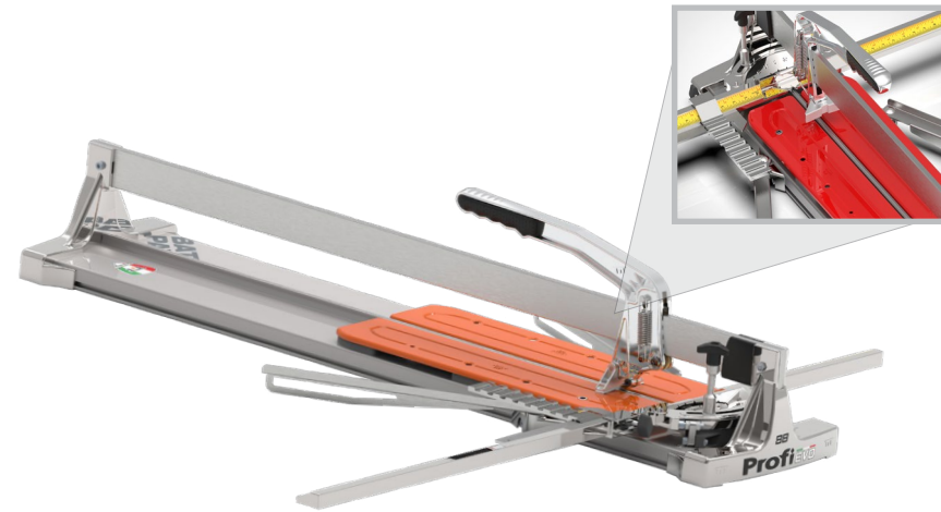
Aluminium draw-plate to get the maximum of rigidity and lightness at the same time.
