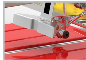
Goniometric square in "90°" position for a direct reading of the measurement for straight cuts (Black lower scale).
